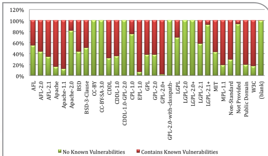
Licenses and Known Vulnerabilities
