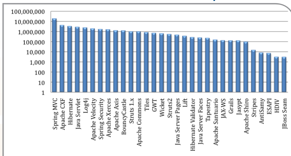
Total Downloads of Each Library
