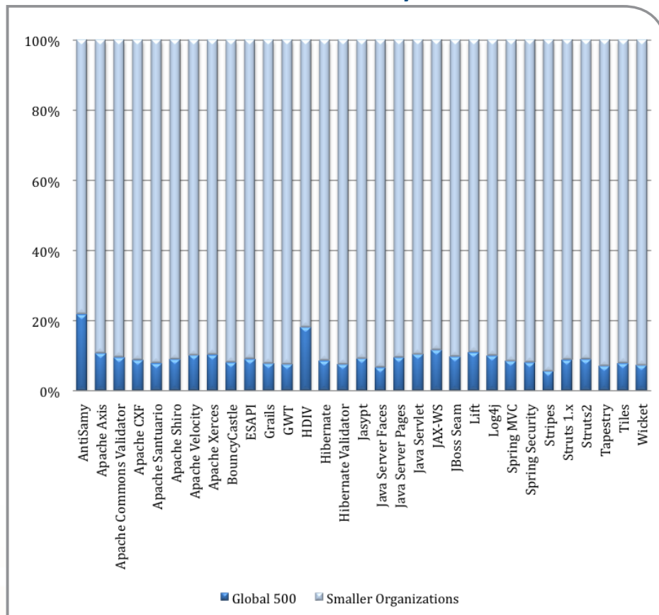
Global 500 Library Use
